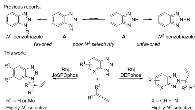
Scheme 2. N -Selective substitution of benzotriazoles.
